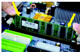
Fig.1 The DIMM socket has a notch, so the DIMM memory module can only fit in one direction. Insert the DIMM memory module vertically into the DIMM socket. Then push it down.
